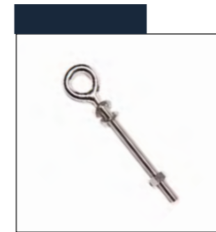
N316-4 M8 x 100 Eyebolt with Nut for wooden pole
