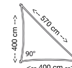
Triangle 90° 4,0 x 4,0 x 5,7m
